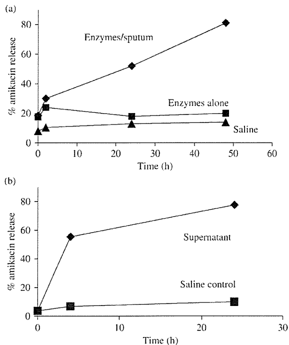
Figure 3. Release of amikacin is mediated by factors produced by biofilm-associated Pseudomonas . (a) Release of amikacin from liposomes in sputum. A sputum sample from a cystic fibrosis patient with a Pseudomonas infection (diamonds) was liquefied enzymatically and amikacin-loaded liposomes were incubated with it at 37°C. Incubation with enzymes alone in saline (squares) or with saline (triangles) alone served as controls. Release of amikacin was measured over time and is expressed as percent maximal. (b) Release of amikacin mediated by a supernatant from a mucoid Pseudomonas biofilm culture. Strain PA3064 was grown for 96 h as a biofilm. The culture was homogenized and clarified by sedimentation. Liposomes were incubated with the supernatant (diamonds) or saline alone (squares) at 37°C and release was monitored as shown.
